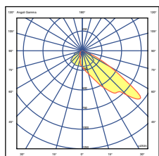
15LED 125W 700mA OTTICA AS
